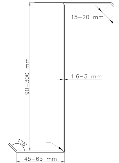
Z Purlin
